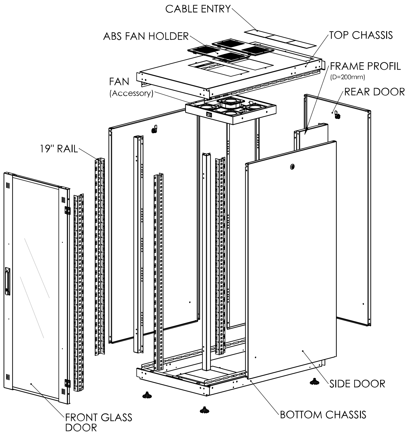
Exploded view
