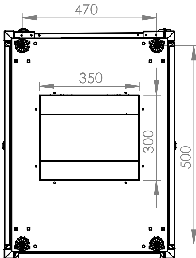
Bottom view
