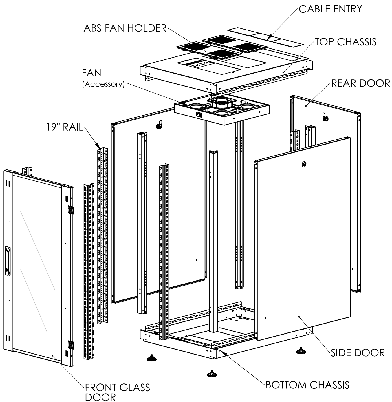
Exploded view
